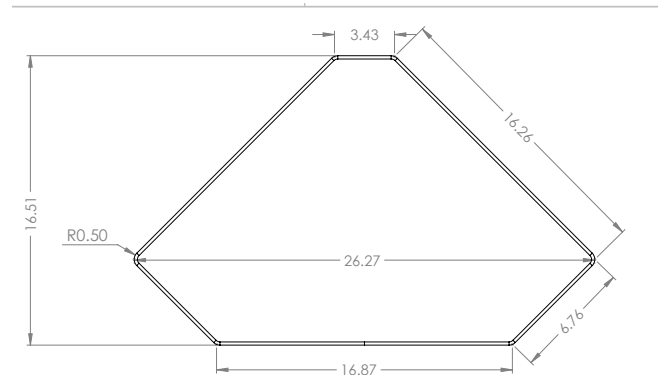
HEXAGON SEAT MAT TOP VIEW
