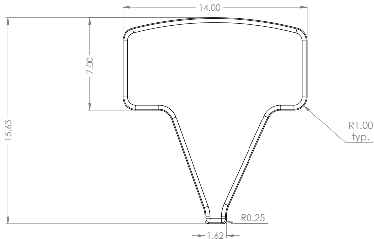
WIT SEAT BACK MAT TOP VIEW
