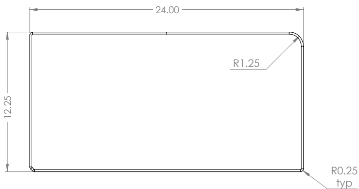
BENCH SEAT MAT TOP VIEW
