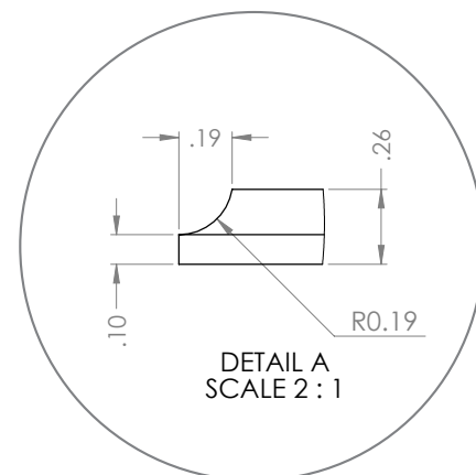
SIDE VIEW - MAGNIFIED
