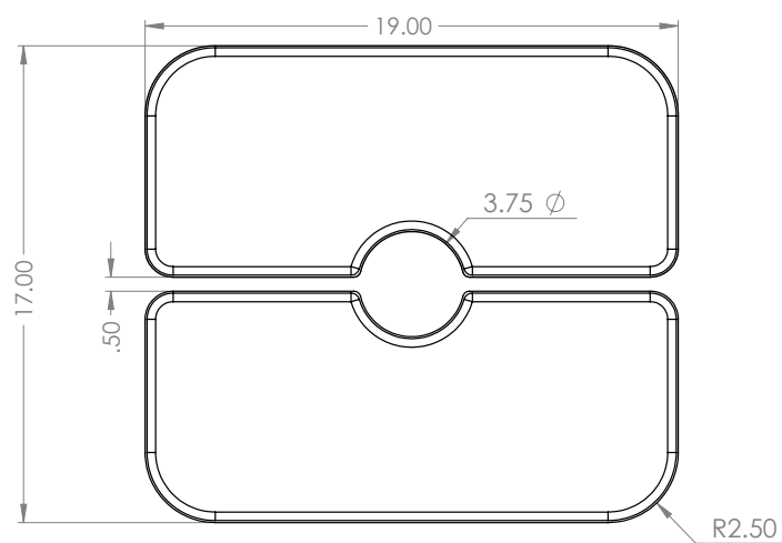
WIT FLOOR MAT TOP VIEW
