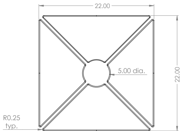
SMALL CENTER DRAIN TOP VIEW
