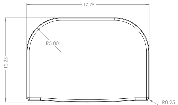
WIT BENCH SEAT TOP VIEW
