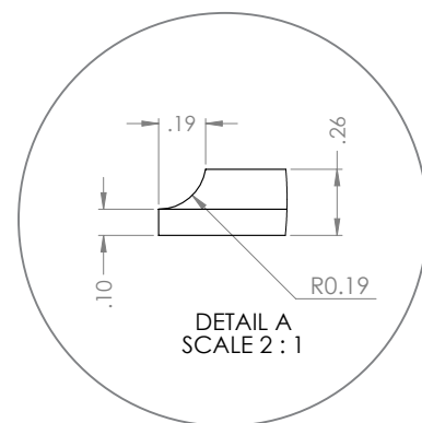
SIDE VIEW - MAGNIFIED
