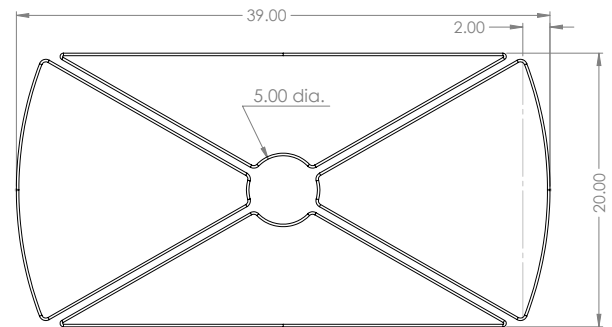
LARGE CENTER DRAIN TOP VIEW
