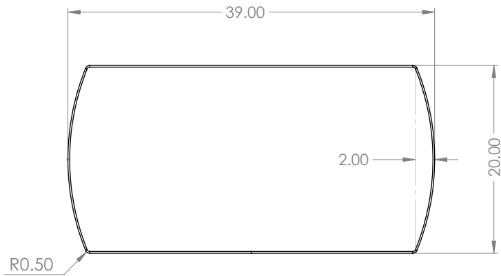
LH/RH DRAIN SHOWER MAT TOP VIEW
