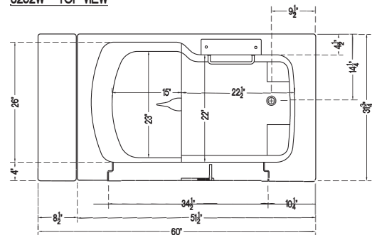
3252W - TOP VIEW
