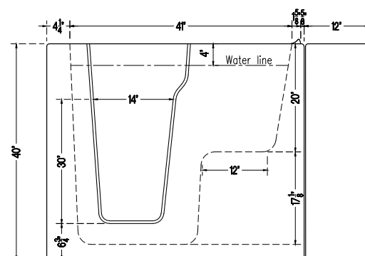
2848 - SIDE VIEW
