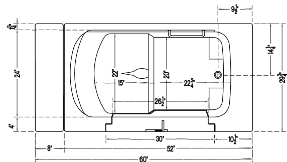
3052W - TOP VIEW
