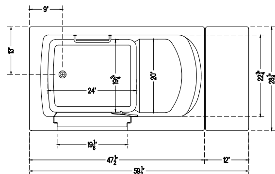
2848 - TOP VIEW
