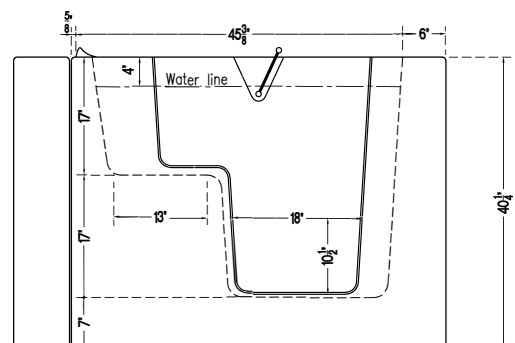
3052W- SIDE VIEW
