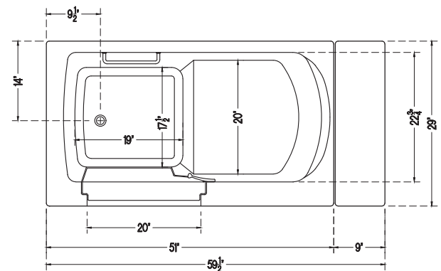
3052-S - TOP VIEW
