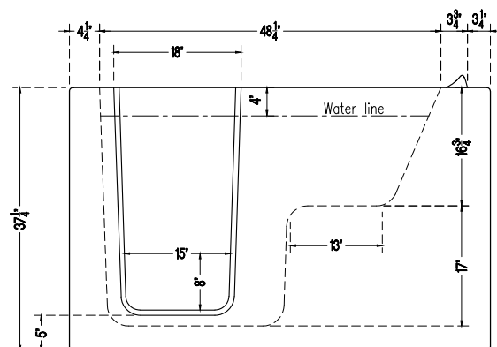
B3060 - SIDE VIEW
