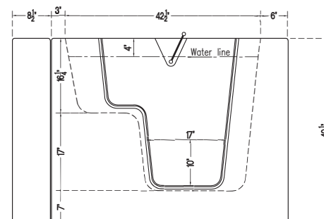
3252W - SIDE VIEW
