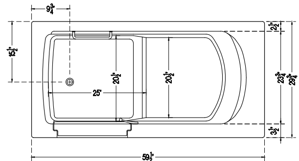
B3060 - TOP VIEW
