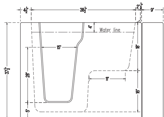
3052-S - SIDE VIEW
